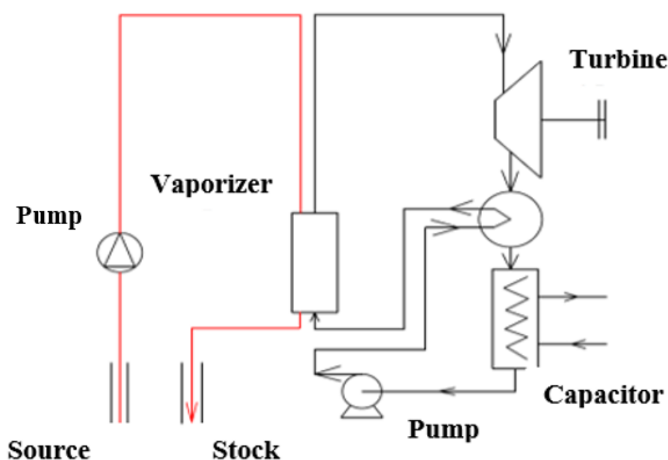
Figure 2. Diagram of an installation with a CRO using geothermal energy
