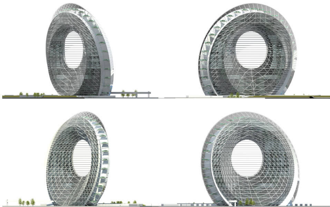
Figure 1. Dutch Windwheel
