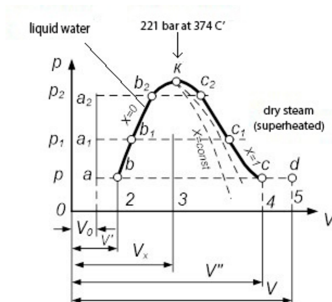
Figure 1. Diagram of water vapor in pressure – volume coordinates
