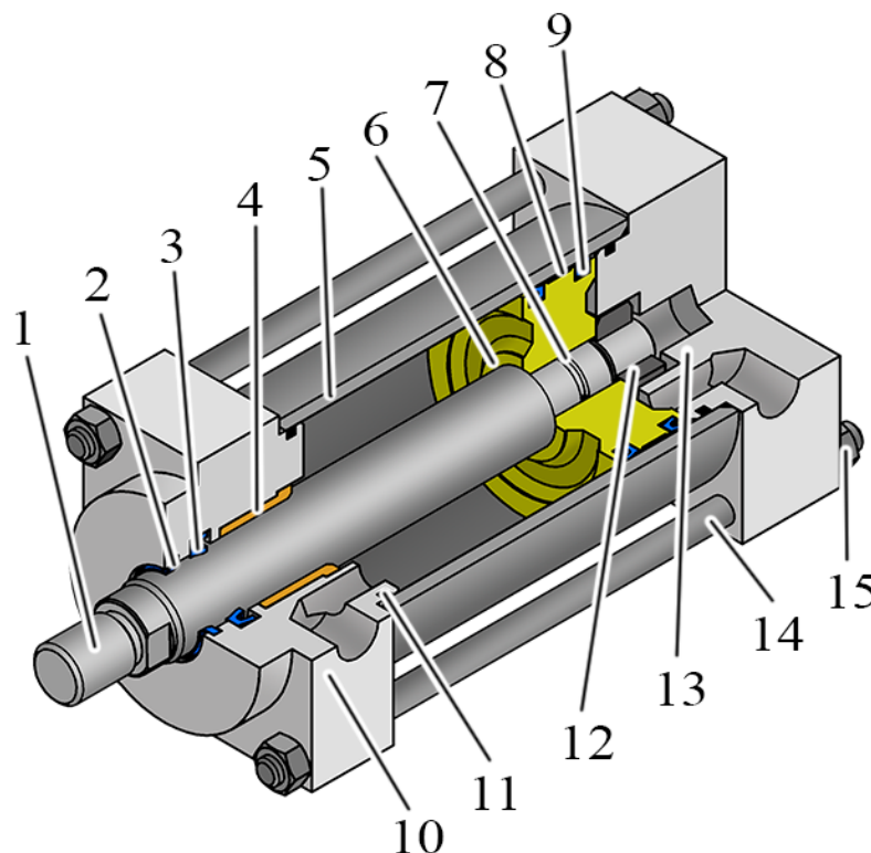
Figure 1. Design of a one-way pneumatic cylinder [3]:
