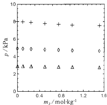
Figure 2. Vapor pressure p of 1,4-dioxane in the 1,4-dioxane + tetrabutylammonium nitrate (2) system: \Delta , 288.15 K; \diamond , 298.15 K; + , 308.15 K. m_2 is the salt molality.
