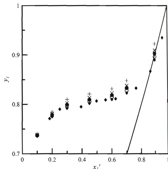
Figure 1. Vapor mole fraction ( y_1 ) of methanol in the methanol (1) + toluene (2) + tetrabutylammonium tetraphenylborate (3) system at T = 318.15 K: \blacklozenge , no salt (Nagata 19 and Kurzin et al. 8 ); \circ , m_3 = 0.100 mol·kg −1 ; \bullet , m_3 = 0.200 mol·kg −1 ; \times , m_3 = 0.300 mol·kg −1 ; + , m_3 = 0.500 mol·kg −1 . The liquid mole fraction of methanol x'_1 is on a salt-free basis. The solid line is to identify the azeotropic behavior.
